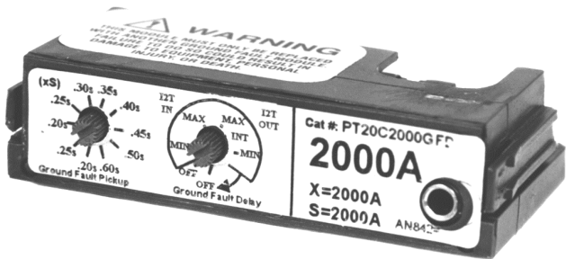
Figure 1. Rating Plug with ground-fault function.
