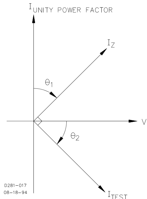
Figure 5-12. Directional Setting
