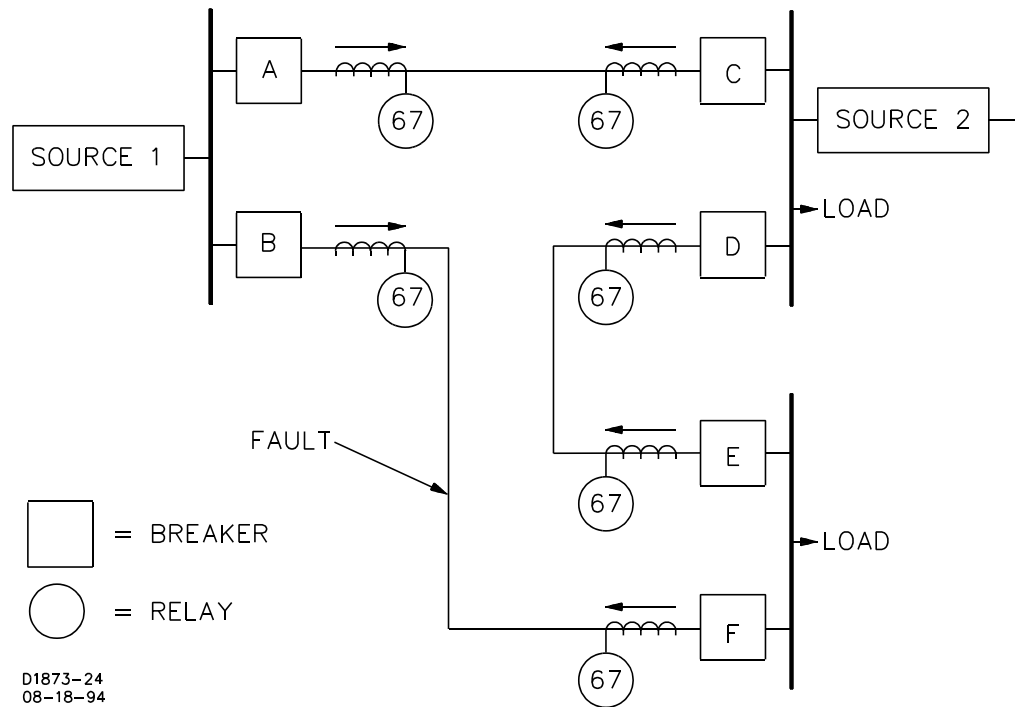
Figure 1-6. Substations Fed From Two Sources
