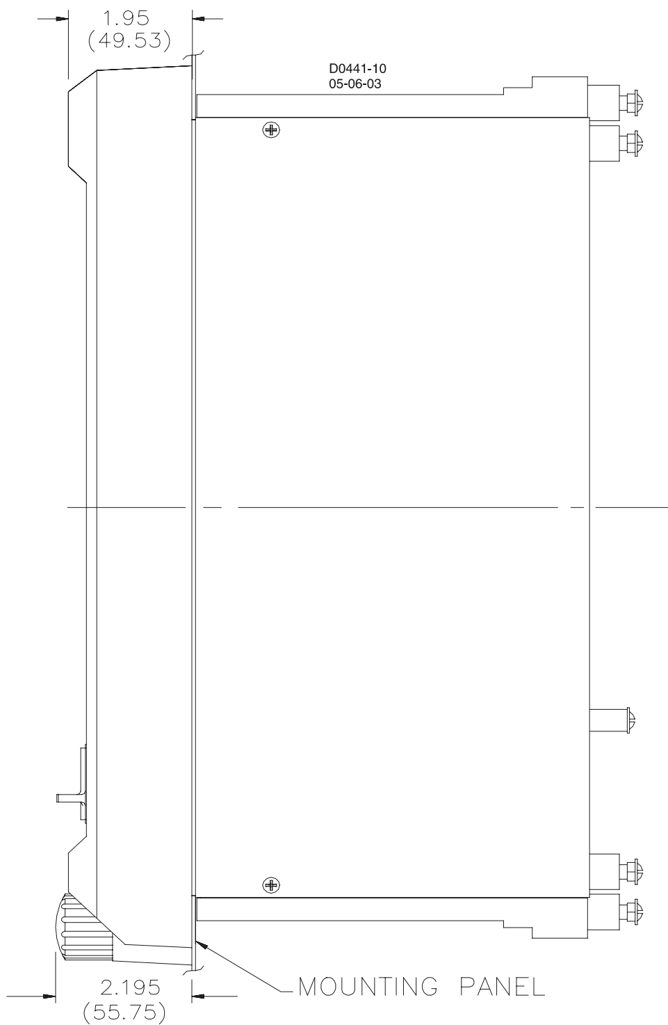
Figure 4-3. Outline Dimensions, Side View — Semi-Flush Mounting
