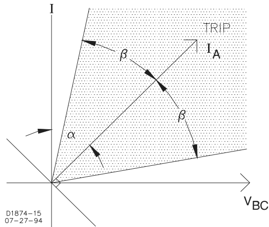
Figure 3-3. Limited Region of Operation
