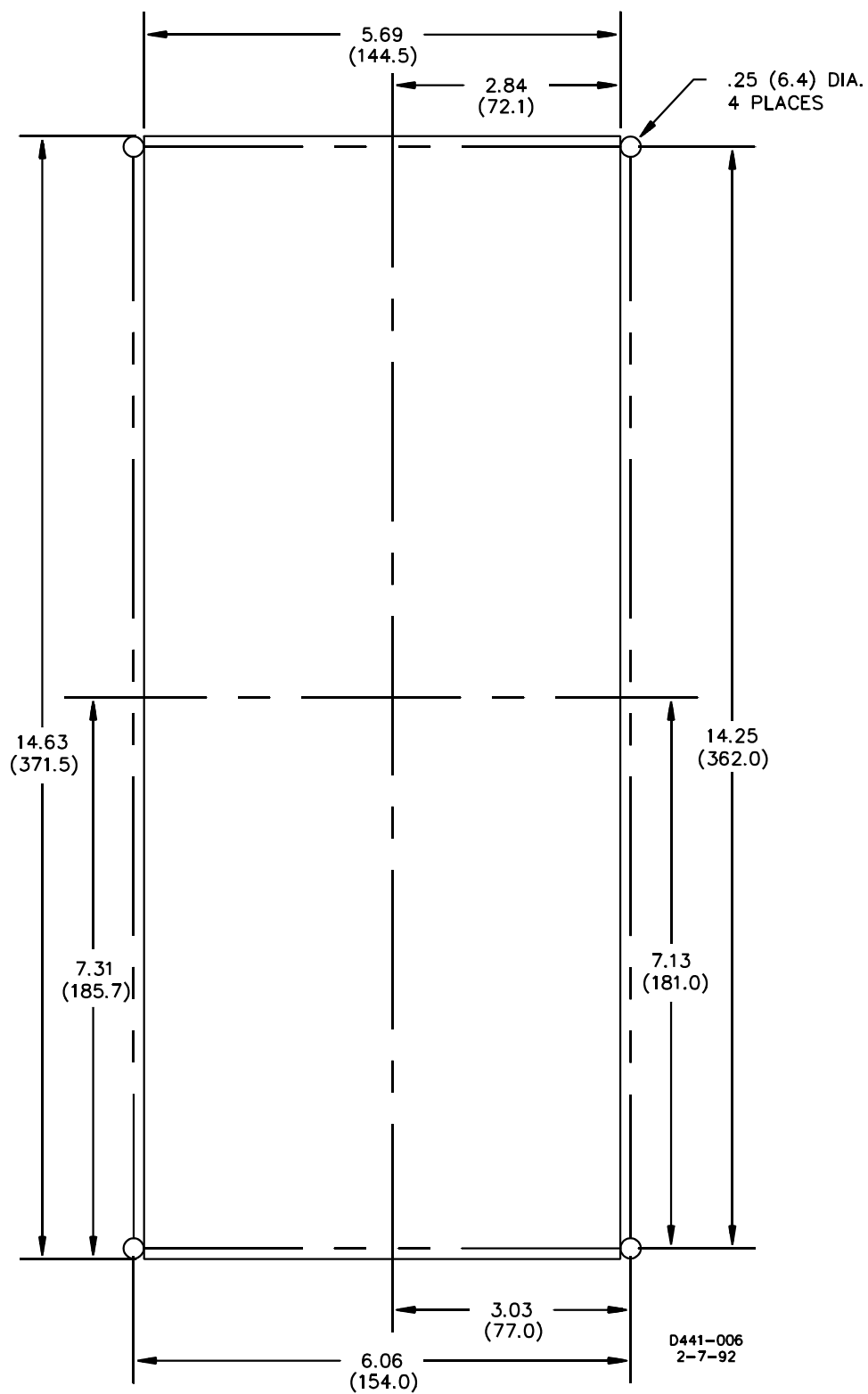
Figure 4-5. Panel Drilling Diagram — Semi-Flush Mounting
