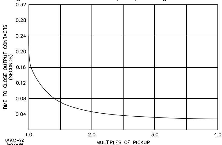
Figure 1-10. Typical Instantaneous Response Time
