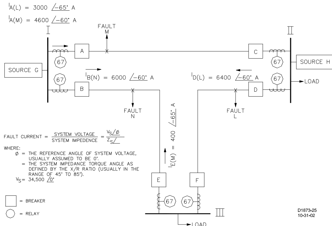
Figure 1-7. Significant Faults for Breaker A
