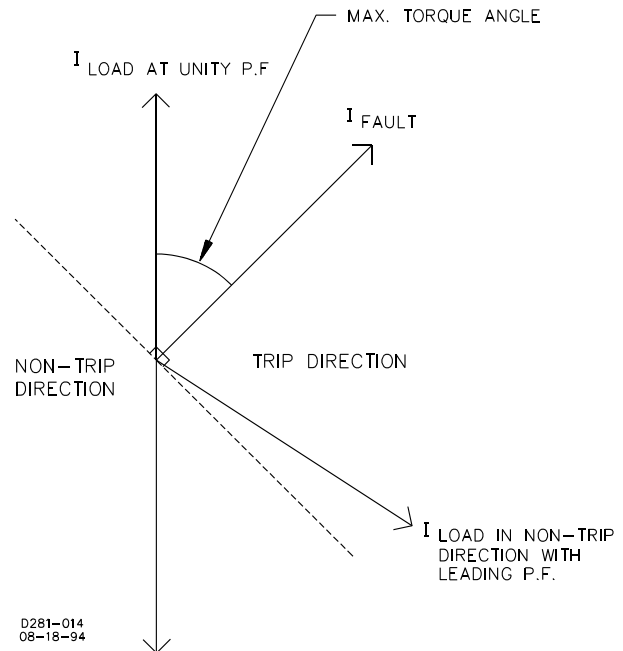
Figure 1-3. Weak Infeed Phenomenon
