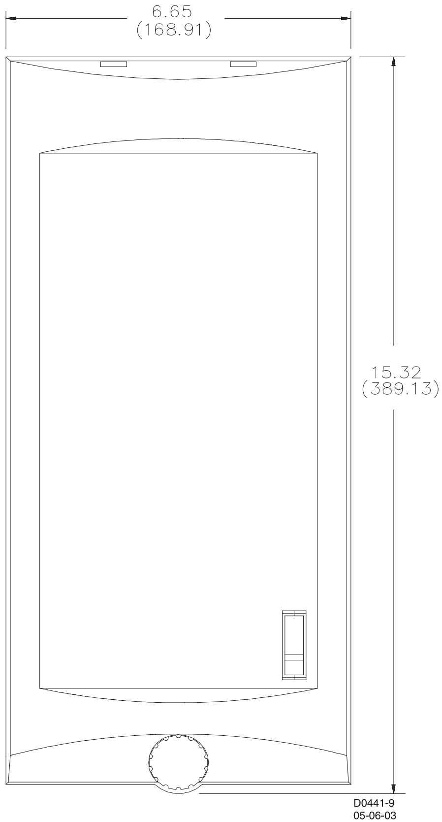
Figure 4-1. Outline Dimensions, Front View
