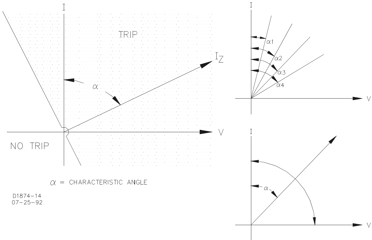
Figure 3-2. Characteristic Angle
