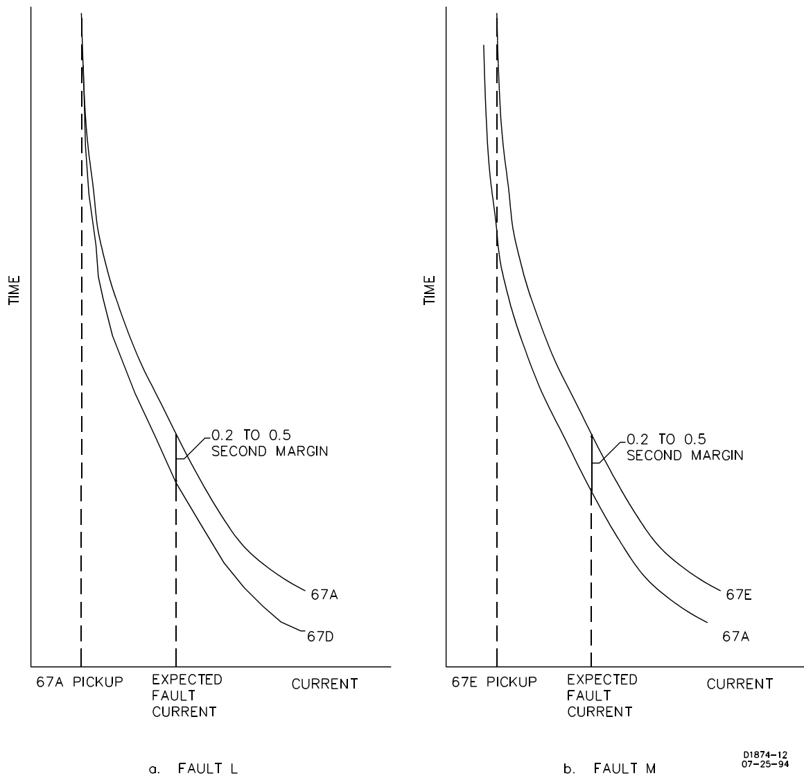
Figure 1-8. Coordination of Time Characteristic Curves
