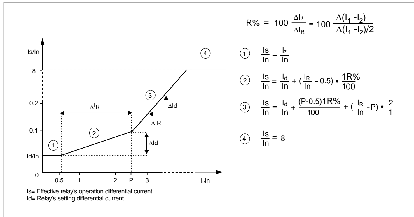
Figure 2. Dual Slope Bias Characteristic of the MD32G Differential Relay
