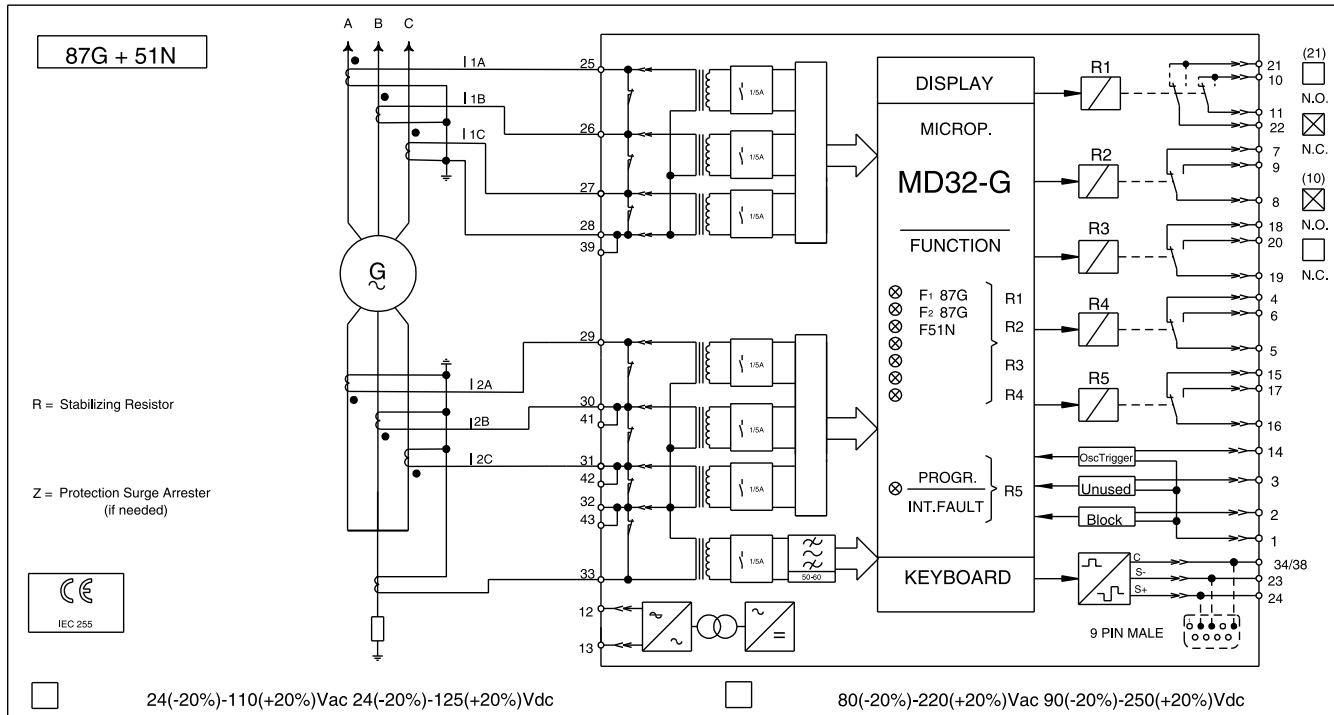
Figure 4. Wiring Diagram for the MD32G Rotating Machine Differential Relay used for 87G and 51N Protection
