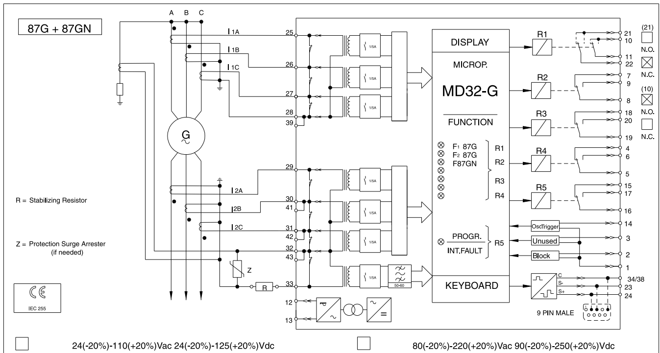
Figure 3. Wiring Diagram for the MD32G Rotating Machine Differential Relay used for 87G and 87GN Protection
