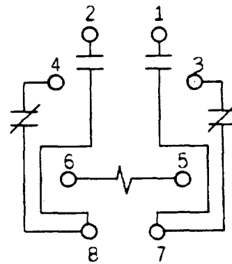
INTERNAL CONNECTIONS (FRONT VIEW)
