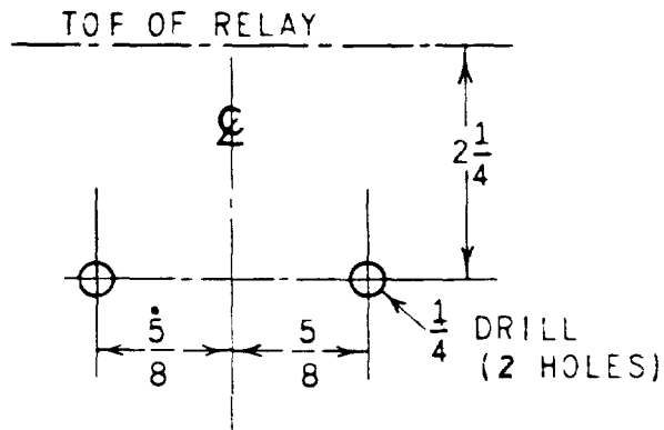
PANEL DRILLING (FRONT VIEW)
