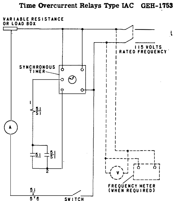
Fig. 18 Testing Connections for Type IAC Relays such as Type IAC51A
