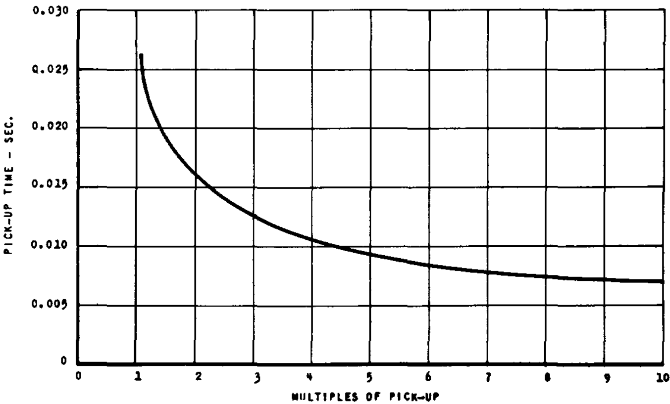
Fig. 10 Time-current Characteristics of Instantaneous Unit
