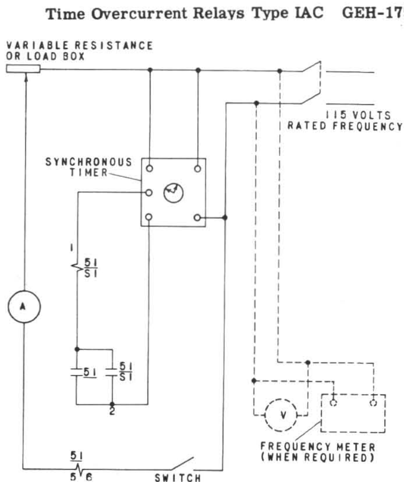
Fig. 18 Testing Connections for Type IAC Relays such as Type IAC51A
