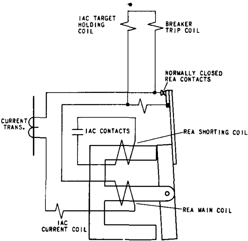
Fig. 9 Diagram Illustrating Operation of Type IAC Relays Having An A-C Tripping Unit
