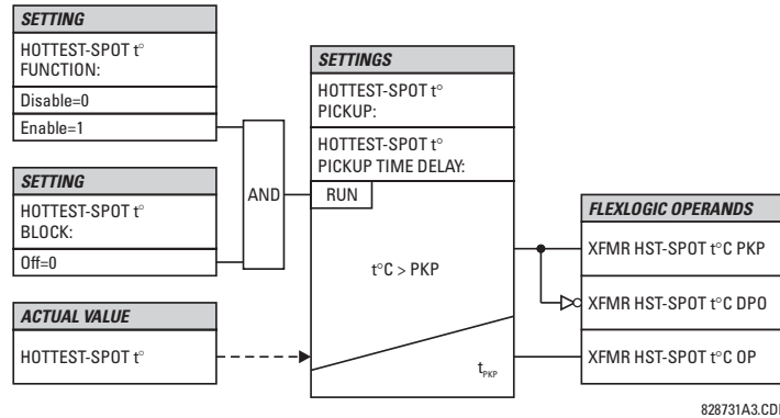
Figure 5-45: TRANSFORMER HOTTEST-SPOT TEMPERATURE LOGIC
