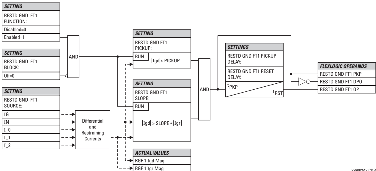
Figure 5-61: RESTRICTED GROUND FAULT SCHEME LOGIC
