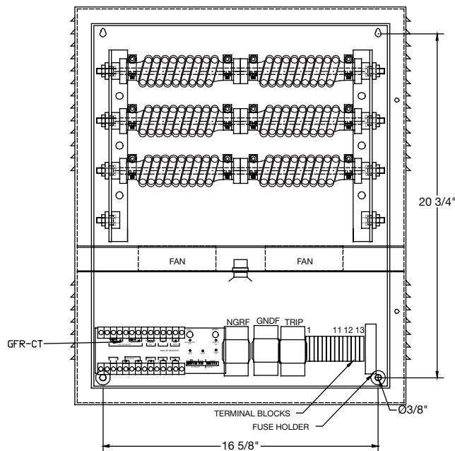
Figure 4 Outside Dimensions
