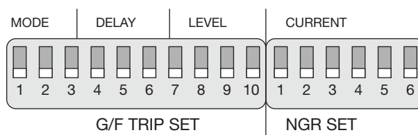
Figure 6 GFR-RM Dipswitch
