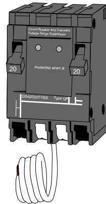
Circuit Breaker and Transient Voltage Surge Suppressor
